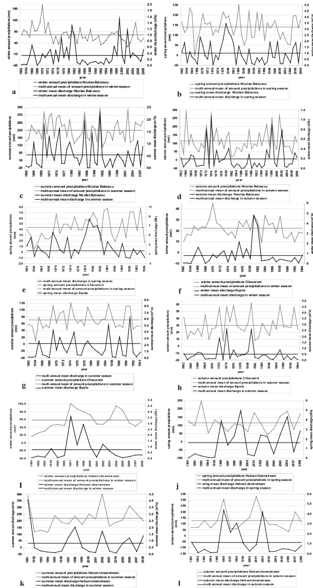
Fig. 4 - Multiannual variation of the annual precipitation amounts (mm) and of the liquid discharges ( \text{m}^3/\text{s} ), at Nicolae Balcescu, in the winter (a), spring (b), summer (c) and autumn (d) (1962–2008); Multiannual variation of the annual precipitation amounts (mm) at Chiscareni, and of the liquid discharges ( \text{m}^3/\text{s} ) at Sipote, in the winter (e), spring (f), summer (g) and autumn (h) (1962–1994); Multiannual variation of the annual precipitation amounts (mm) and of the liquid discharges ( \text{m}^3/\text{s} ), at Halceni–downstream, in the winter (i), spring (j), summer (k) and autumn (l) (1991–2008).
