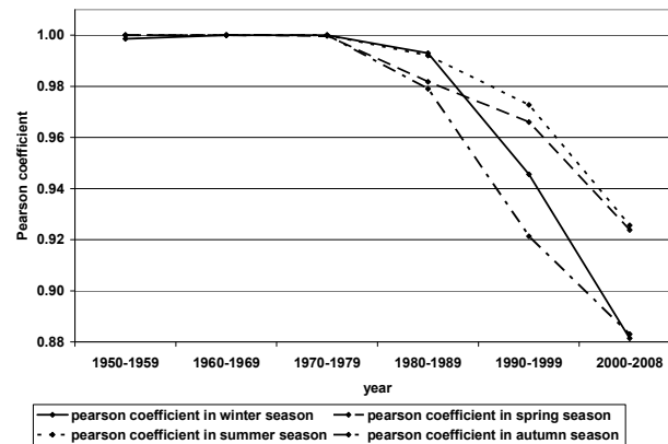
Fig. 6 - Seasonal variation of Pearson's correlation coefficient that characterizes the liquid discharges at the rainfall stations with natural runoff (Nicolae Balcescu and Sipote), in the Miletin River basin, in the period 1950–2008
