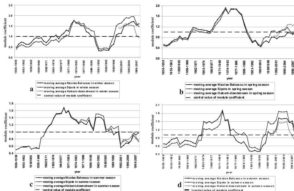
Fig. 5 - a. Evolution of module coefficients, calculated with moving averages every 10 years, staggered by a year in the winter, spring, summer and autumn, in the Miletin hydrographic basin (1950–2008)
