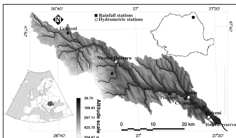
Fig. 1 - Geographic location of the Miletin hydrographic basin and position of hydrometric stations
