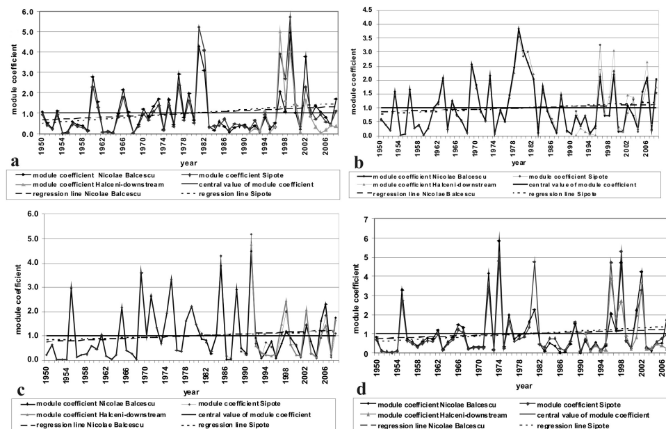
Fig. 3 - Multiannual variation of module coefficients, during the winter (a), spring (b), summer (c) and autumn (d), in the Miletin River basin (1950–2008)
